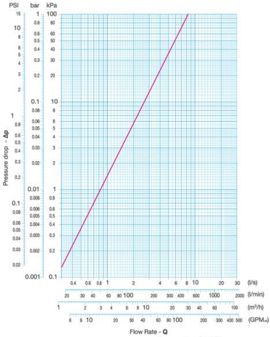
Pressure Loss Data Diagram
