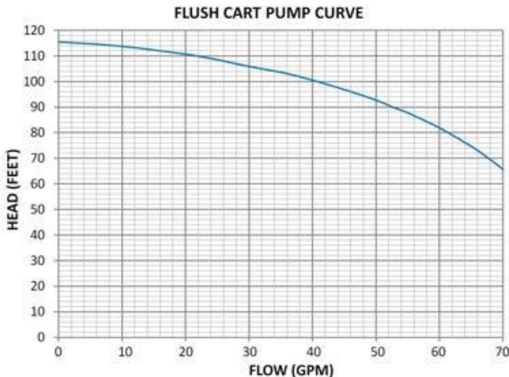
Figure 1: Munro LP Series performance curve
