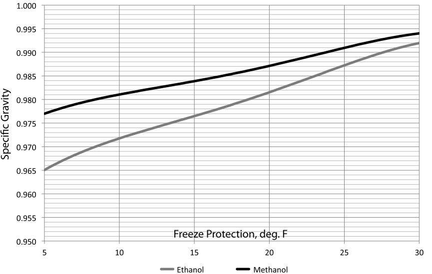
Figure 17: Specific gravity for alcohol-based antifreezes over a range of freeze protection temperatures (source: Geo-Flo Calculator apps, www.geo-flo.com )
