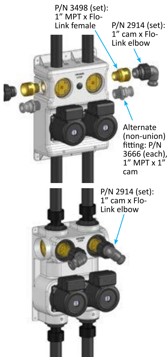
Figure 4: FPT flow center (top) and Flo-Link Double O-ring flow center (below) flush cart fittings
