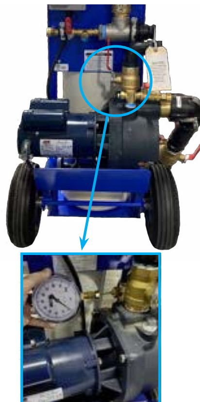
Figure 19: Measuring pressure drop
