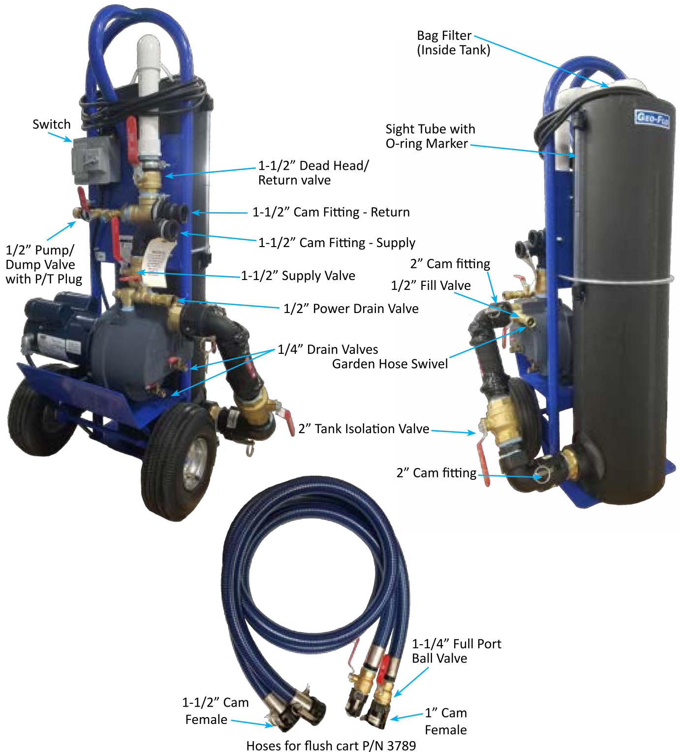
Figure 2: Flush cart diagram with descriptions
