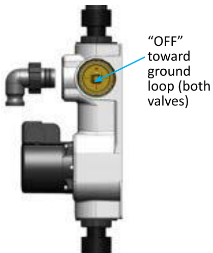
Figure 9: FPT flow center (top) and Flo-Link Double O-ring flow center (below) valve positions for ground loop isolation
