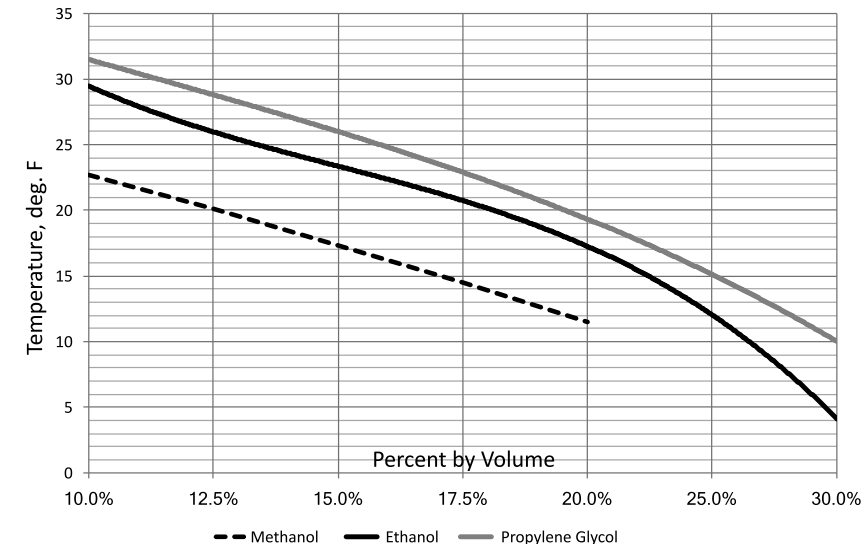
Figure 16: Freeze protection for common ground loop antifreeze mixtures (source: Geo-Flo Calculator apps, www.geo-flo.com )
