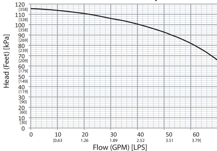
Flush Cart Munro Pump Curve
